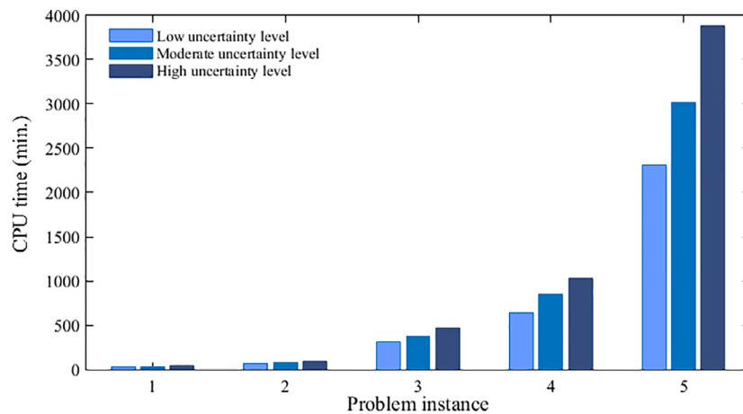
Fig. 6. Impact of uncertainty level on required CPU time in hybrid simulation-analytical modeling approach.
