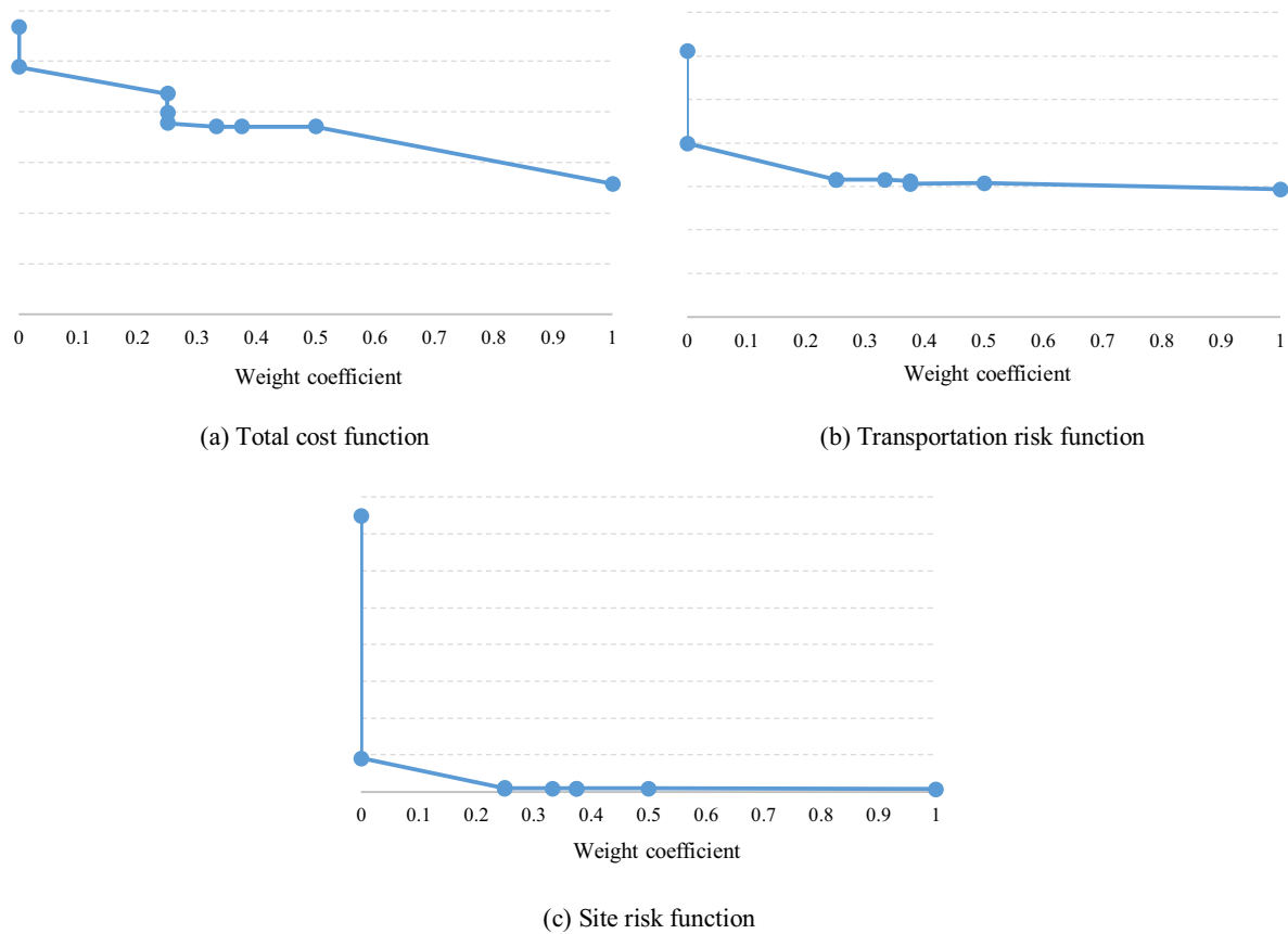
Fig. 13. Trend of objective functions under different weight coefficient combination scenarios.
