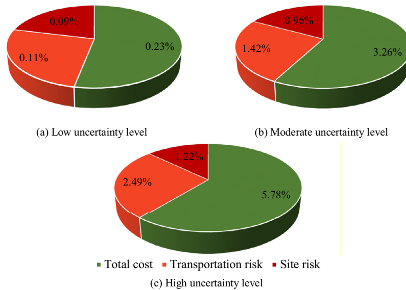
Fig. 5. Uncertainty impact under different uncertainty scenarios.
