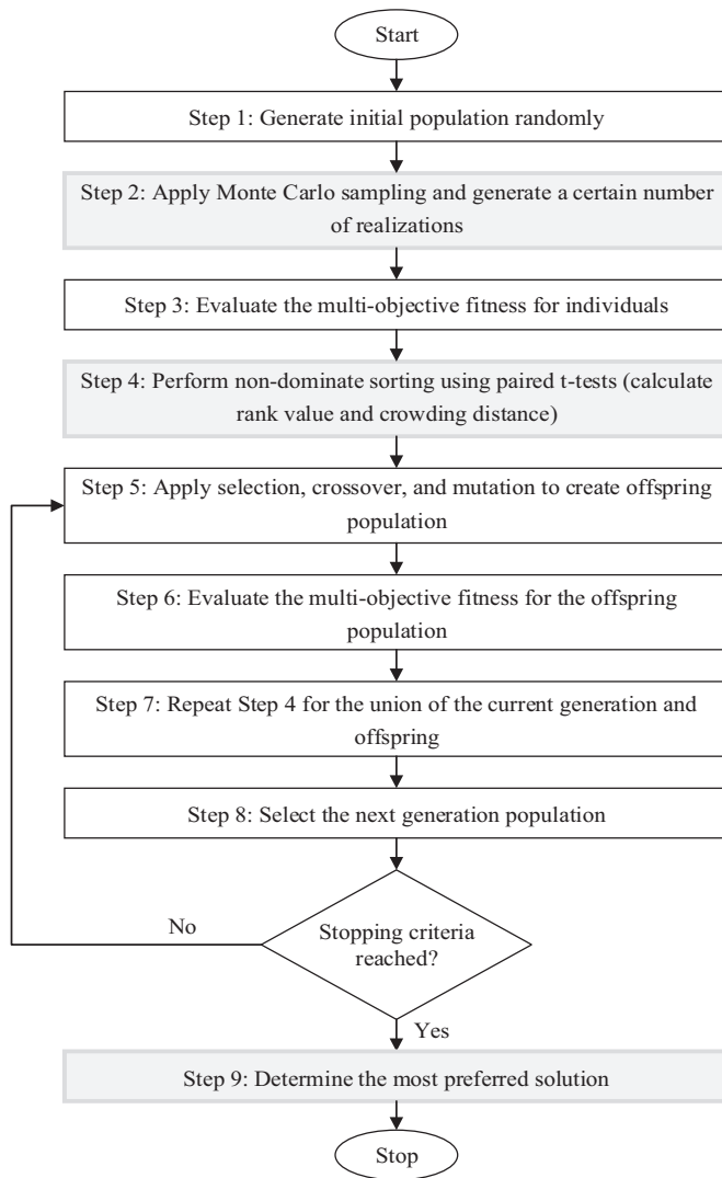
Fig. 2. Flowchart of the proposed simheuristic algorithm.
