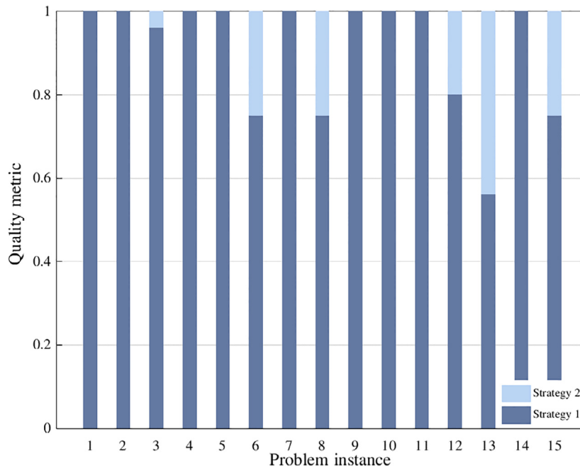
Fig. 11. Quality metric under different solution comparison strategies.
