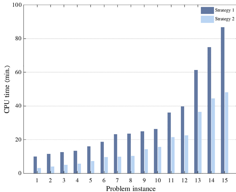
Fig. 10. Required CPU time under different solution comparison strategies.
