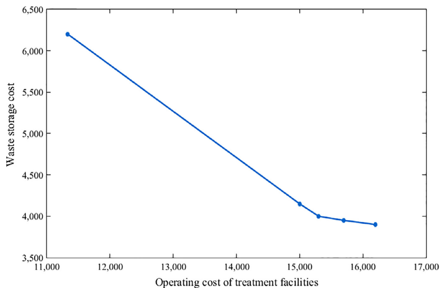
Fig. 14. Conflicting nature of operating and waste storage costs in treatment facilities.
