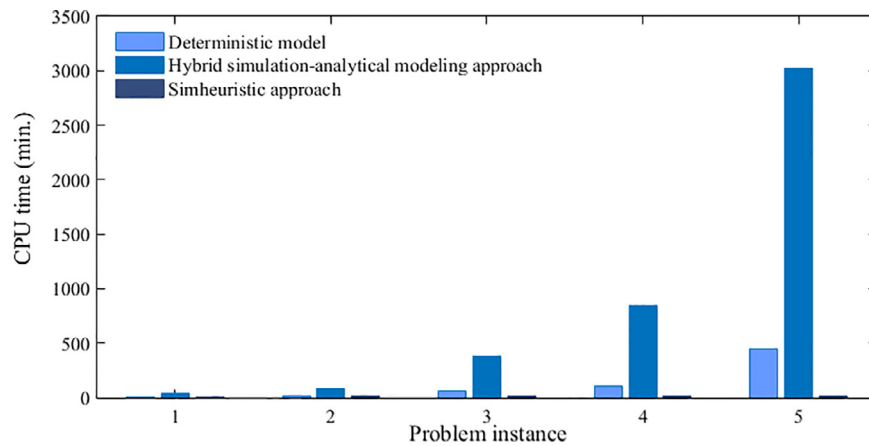
Fig. 7. Required CPU time for solving the small-scale problems with moderate uncertainty level.
