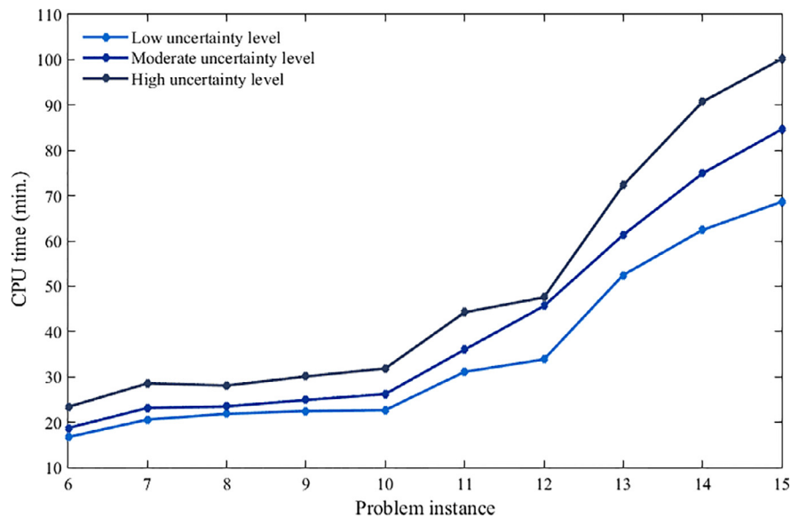
Fig. 9. Required CPU time for medium and large-size problems.
